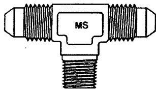
AN825 (MS20825) FLARE TO PIPE TEE
