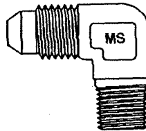
AN822 (MS20822) ANGLE - PIPE TO FLARE
