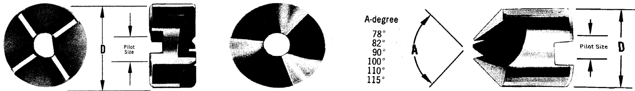
MM280 Reverse Spotfacer 4 Flute
